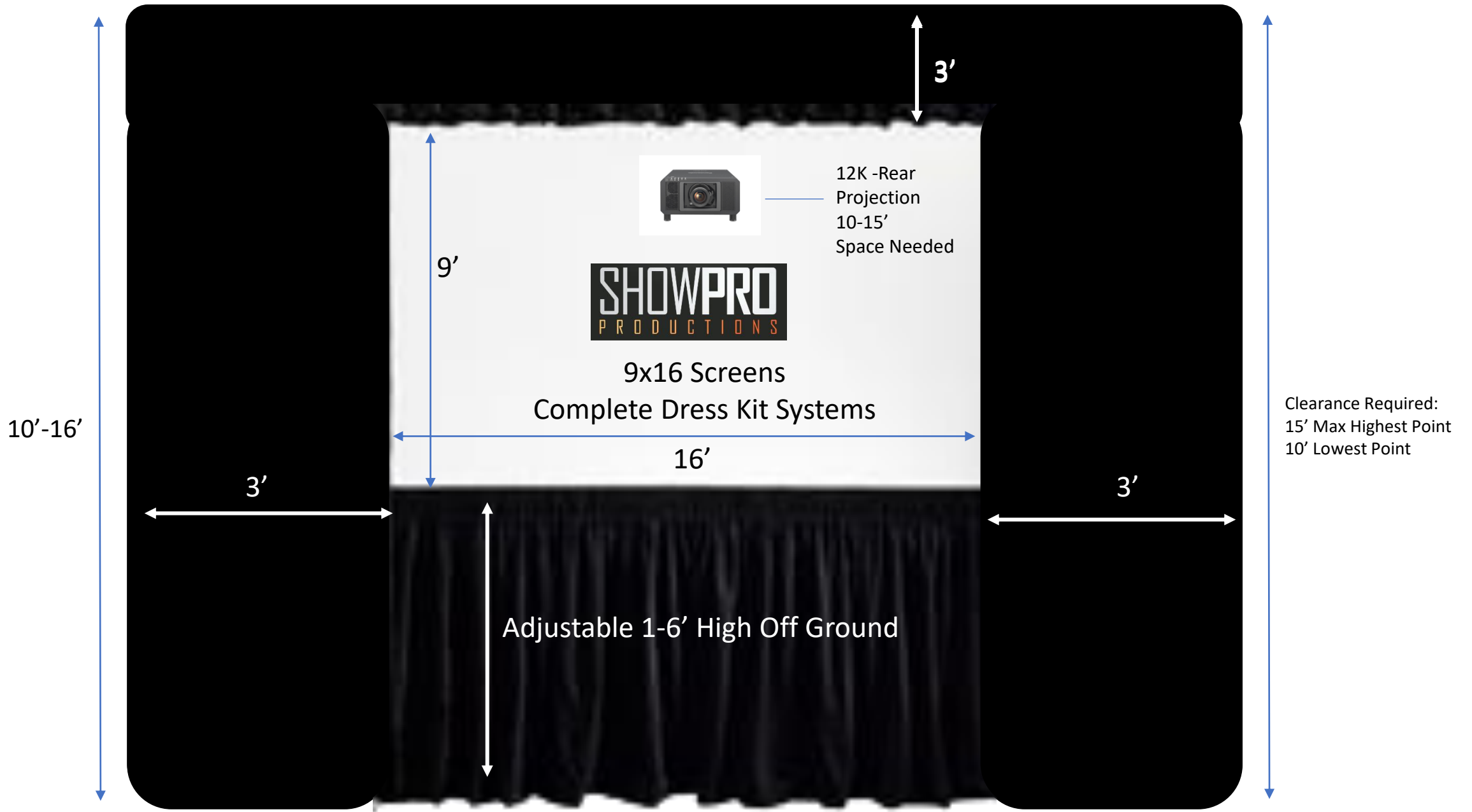
ShowPRO Fast Fold Screen Size
